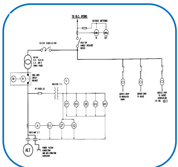
Electrical Single Line Diagram
