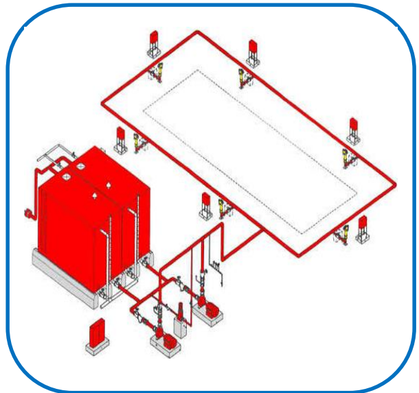
Fire Hydrant & Sprinkler System
